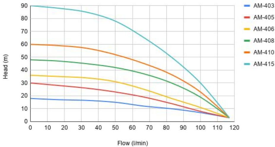
Performance Curve - AM Series
