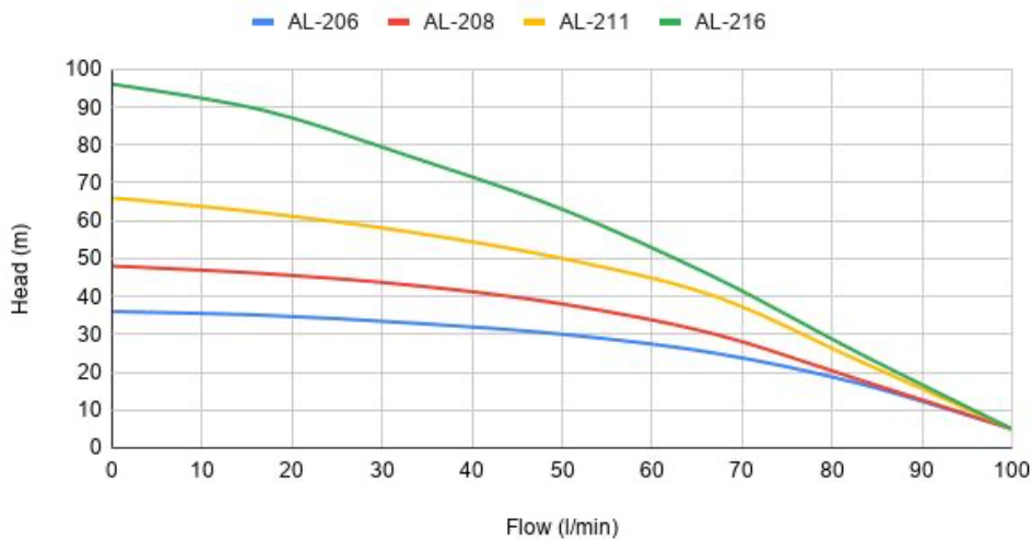
Performance Curve - AL Series
