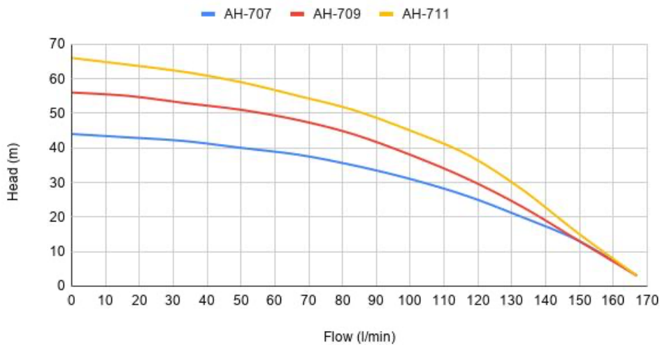
Performance Curve - AH Series
